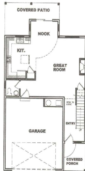
766 SQ' MAIN FLOOR
